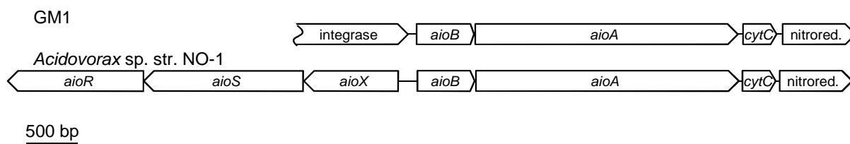
Fig. 1 Arrangement of the aio gene clusters in GM1 and the putative arsenite oxidiser Acidovorax sp. str. NO-1. 19 aioR : encodes response regulator; aioS : encodes sensor histidine kinase; aioX : encodes arsenite-binding protein; aioA : encodes arsenite oxidase large catalytic subunit; aioB : encodes arsenite oxidase small subunit; cytC : encodes putative c -type cytochrome. Acidovorax sp. str. NO-1 accession number: HM357240.1.
